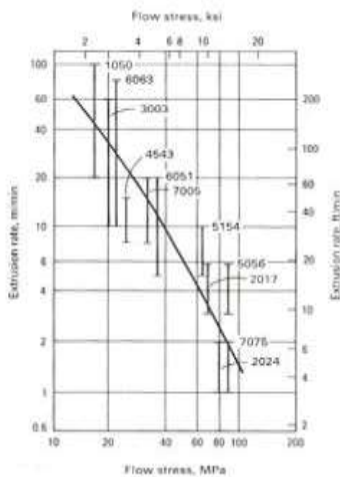
Figure 3: Extrusion rate versus flow stress
