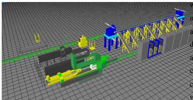
Figure.6 The IGRIP model of the extrusion
