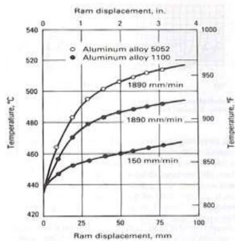
Figure 4. Surface temperature of extruded Product versus ram displacement
