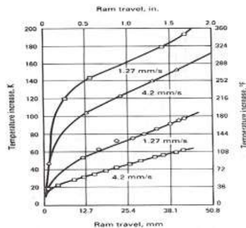
Figure 5. Increase in emergent temperature
