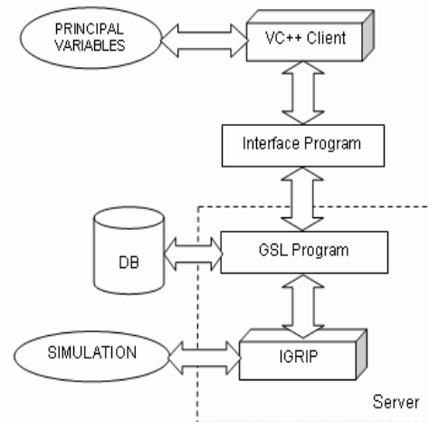
Figure 7. The implementation architecture
